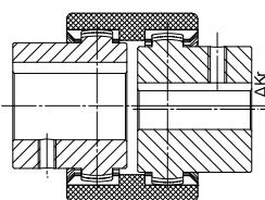
radial misalignment
