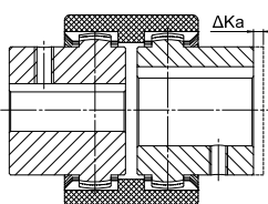
axial misalignment
