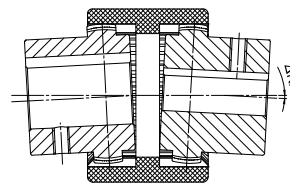
angular misalignment
